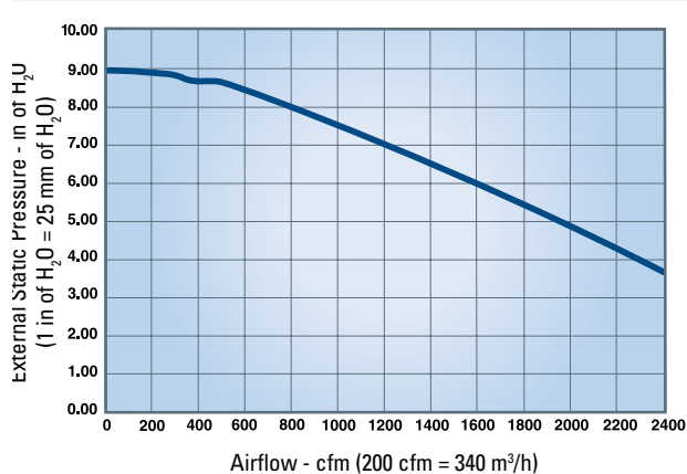
DFO 3-3 4.0kW 50Hz with 9" (228.6 mm) inlet duct (clean filters)
