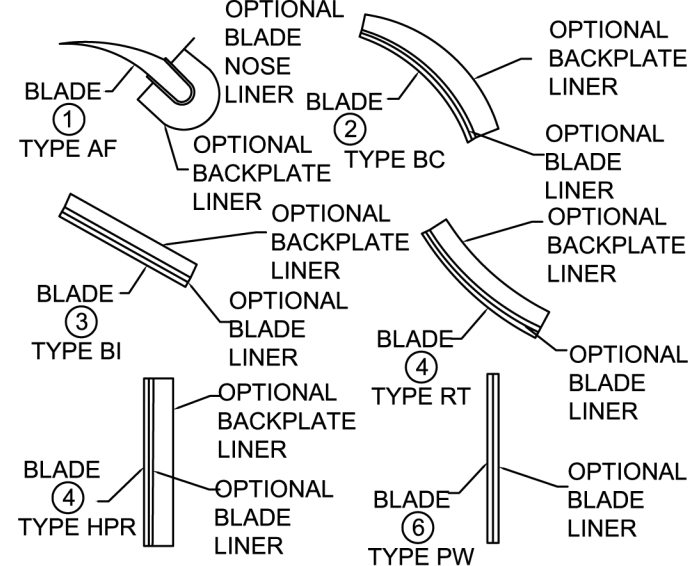
TYPICAL BLADE, BLADE NOSE & BACKPLATE LINERS
