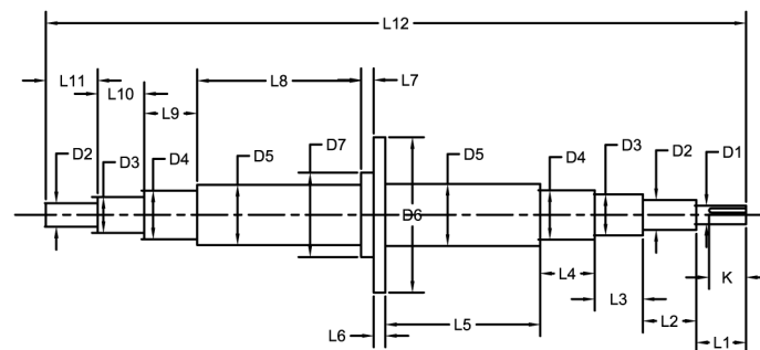
SHAFT DIMENSIONS DOUBLE WIDTH
